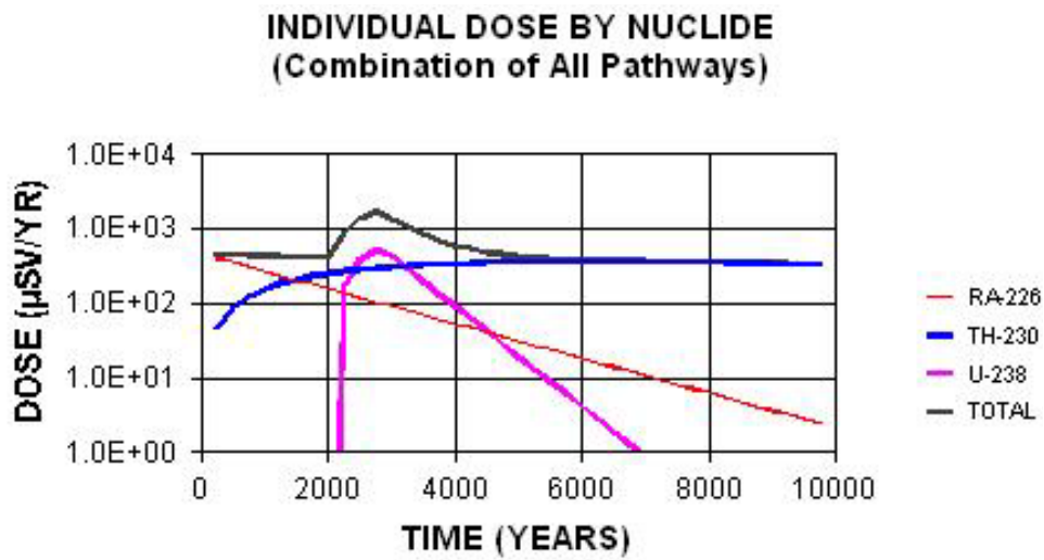
Fig. V.22. PRESTO results for each nuclide for covered waste (2 m of cover).
