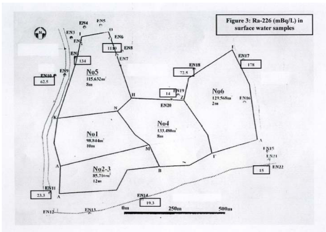
Fig. VII.6. Distribution of 226 Ra concentrations in surface water.
