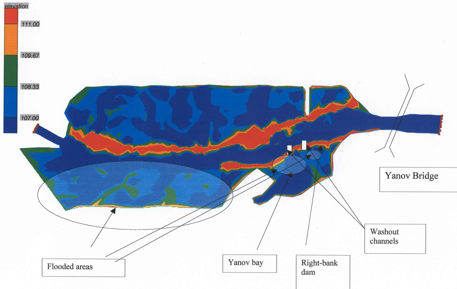
Fig. 3. Scheme of the Pripjat River floodplain area in 1999.
